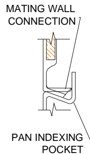
DETAIL F - SCALE: NTS PAN JOINT DETAIL
